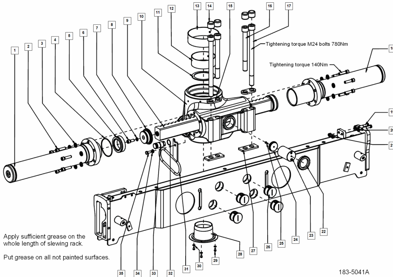
1835041 - Slewing group assembly (s/n 066 0742 and up)
